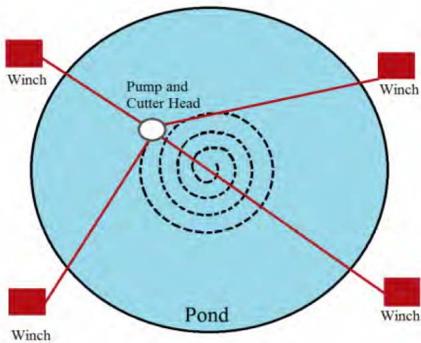
Standard Dredge Pattern
